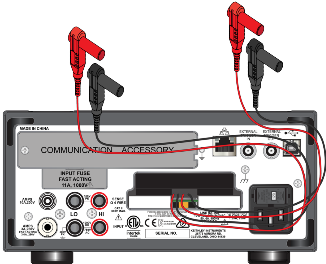
Figure 38: DMM6500 rear panel with TCSCAN card
