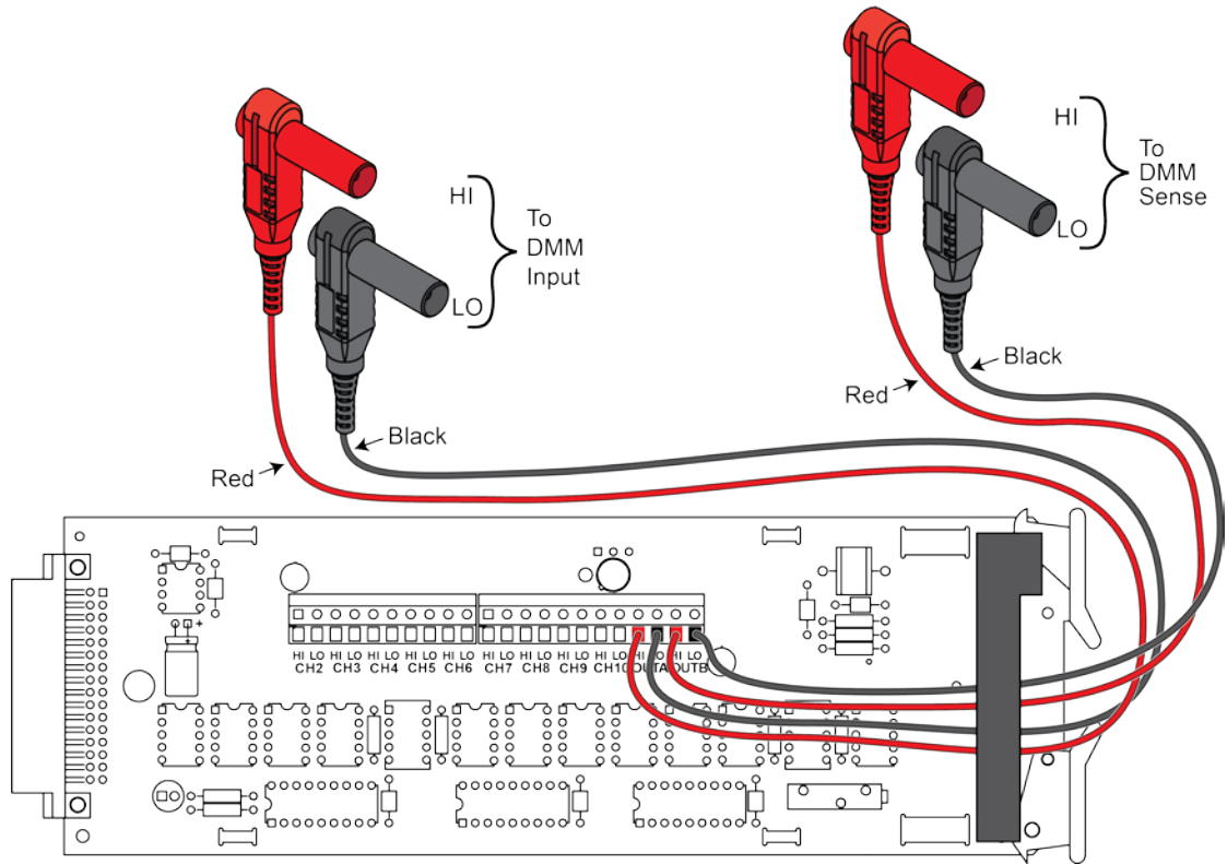
Figure 37: 2001-TCSCAN card
