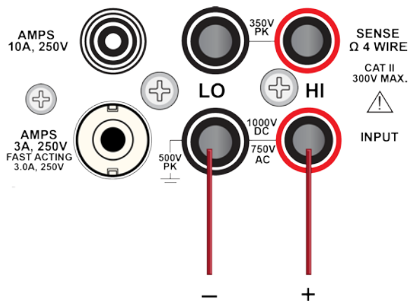
Figure 32: Rear-panel connections
