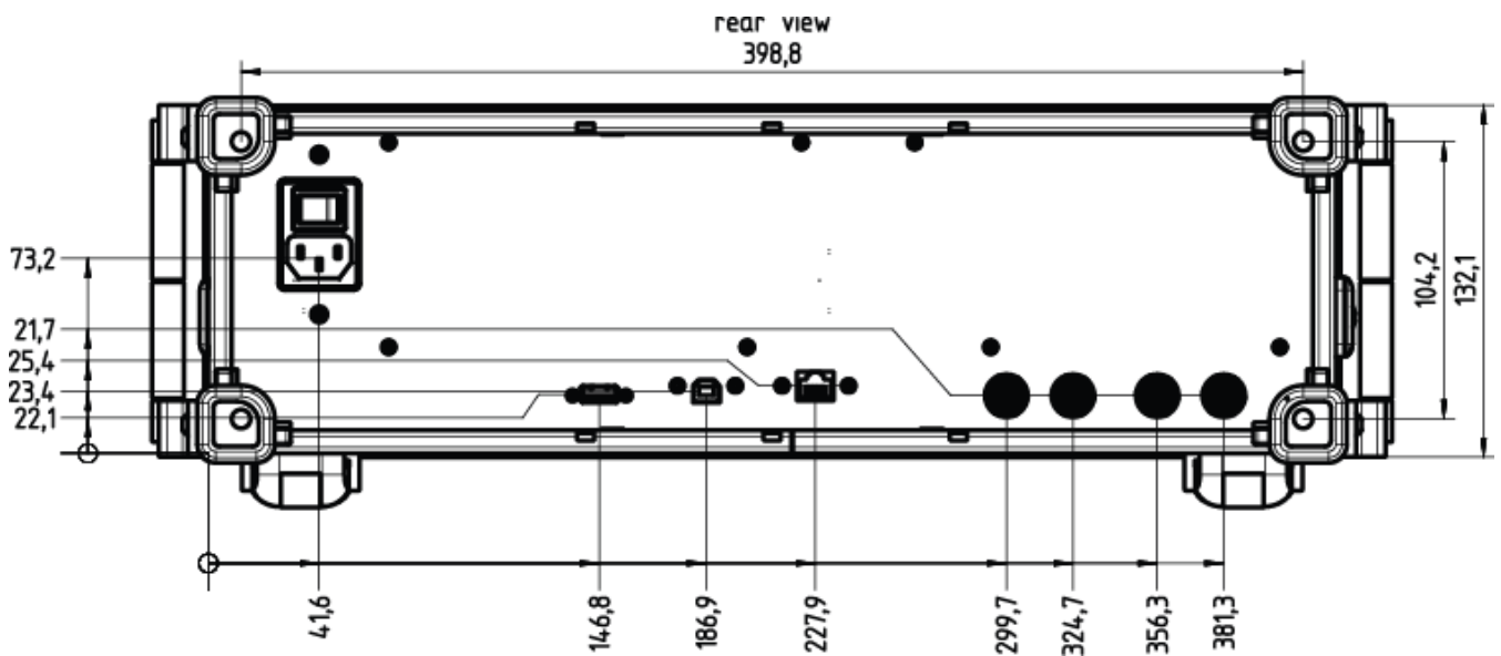
Rear view of the R&S®ZVAX-TRM.
