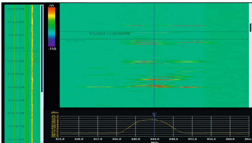
Long time spectrogram recording analysis with R&S®FSH4View.
