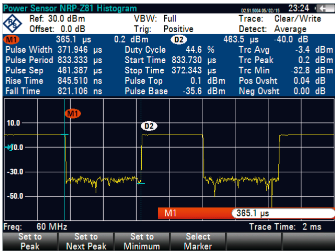
Pulse analysis with R&S FSH-K29 and R&S NRP-Z81 wideband power sensors.
