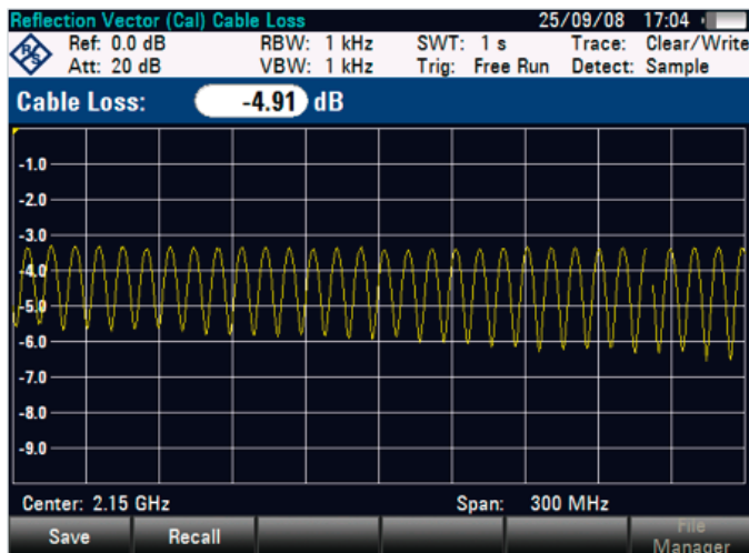
Cable loss measurement.
