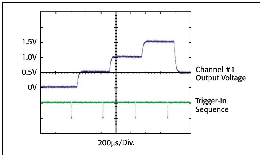
Figure 1. This graph illustrates Channel #1 output voltage response times based on a four-point voltage step sequence (0.5V/1.0V/1.5V/0.5V). The Model 2306-VS can complete this sequence within 1.5ms.
