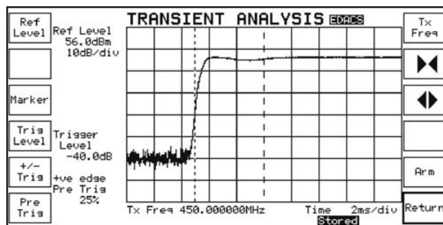
Transient power analysis showing the same bad radio with the 300 kHz IF filter
