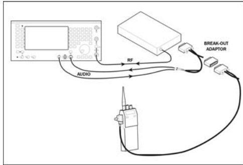
Automatic test connections
