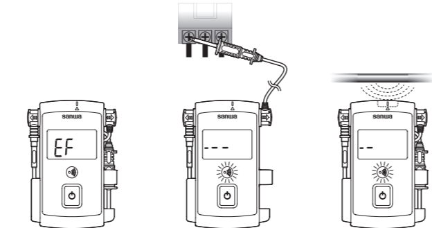
Backlight: Green Undetected status Backlight: Orange Detected status (Contact type) Backlight: Orange Detected status (Noncontact type)
