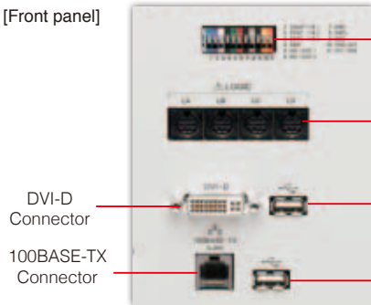
[Front panel]
