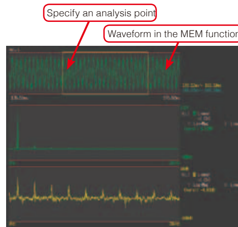
Source waveform (captured in Memory function), and FFT analyzed waveform display simultaneously
